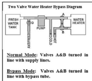
Two Valve Water Heater Bypass
